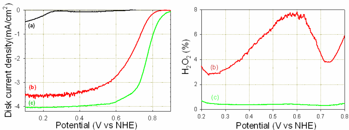
Figure 2. ORR activity and \text{H}_2\text{O}_2 yield obtained with PANI-FeCo-C catalyst at different catalyst synthesis stages (a) before pyrolysis; (b) after pyrolysis but before chemical treatment; (c) after chemical treatment.
