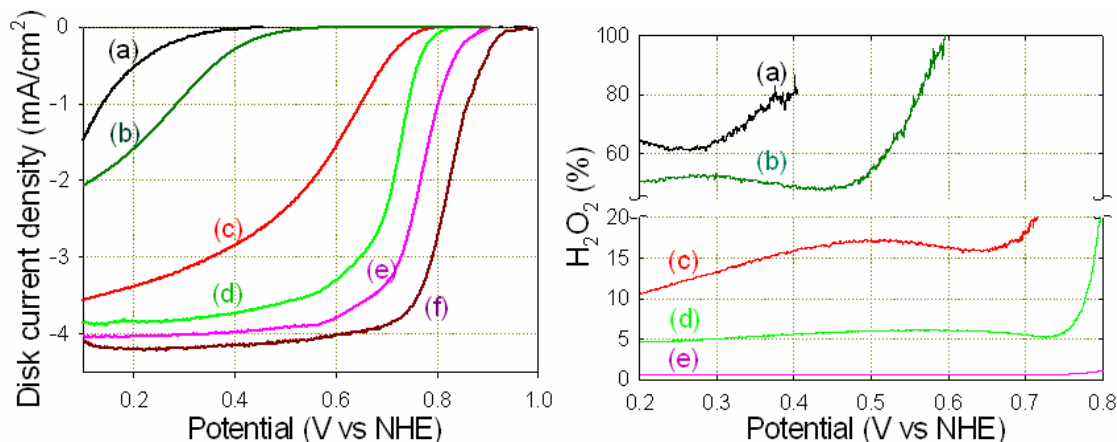
Figure 1. RDE polarization plots (left) and RRDE H 2 O 2 yields (right) recorded with various catalysts in 0.5 M H 2 SO 4 : (a) as-received carbon black; (b) pyrolyzed carbon black; (c) PANI-C; (d) PANI-Co-C; (e) PANI-FeCo-C; (f) E-TEK Pt/C catalyst (Pt loading: 0.06 mg cm -2 ). See Experimental Details for additional information.
