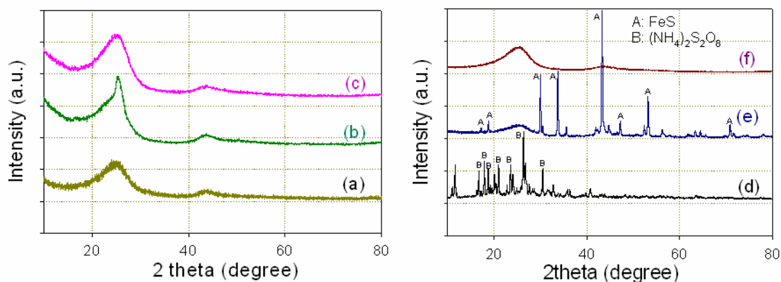
Figure 8. XRD patterns for various support/catalyst samples: (a) as-received carbon black; (b) pyrolyzed carbon black; (c) PANI-C; (d) PANI-Fe-C, before pyrolysis; (e) PANI-Fe-C, after pyrolysis but before chemical treatment; (f) PANI-Fe-C, after chemical treatment.
