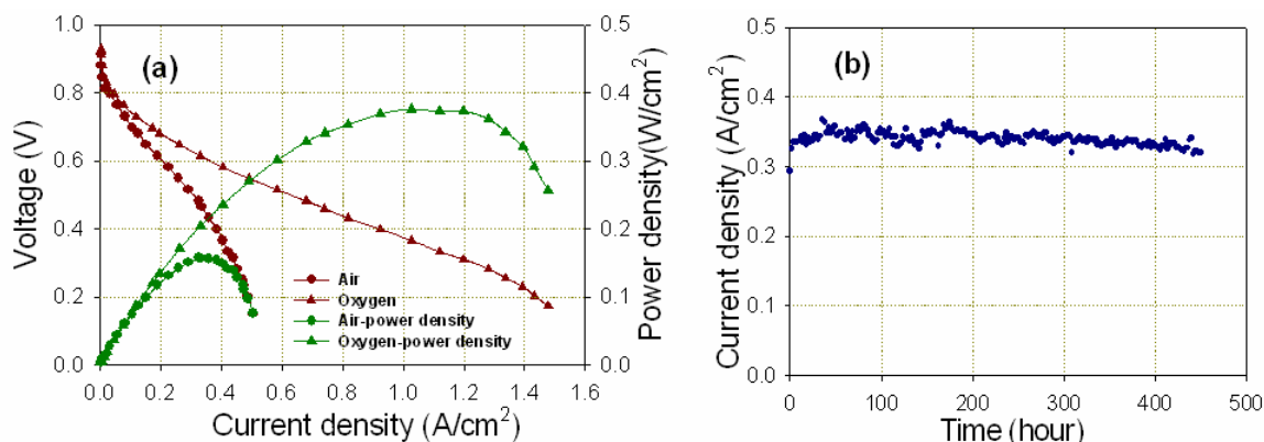
Figure 4. Fuel cell testing of a PANI-FeCo-C cathode catalyst at a loading of 4 \text{ mg cm}^{-2} ; cathode backpressure of 30 psig and 80^\circ\text{C} (a) polarization curves; (b) life test at 0.40 V using \text{H}_2/\text{Air} .
