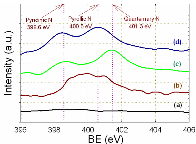
Figure 6. N 1s spectra of XPS analysis for (a) carbon; (b) PANI-coated carbon; (c) PANI-C catalysts; (d) PANI-FeCo-C catalysts.
