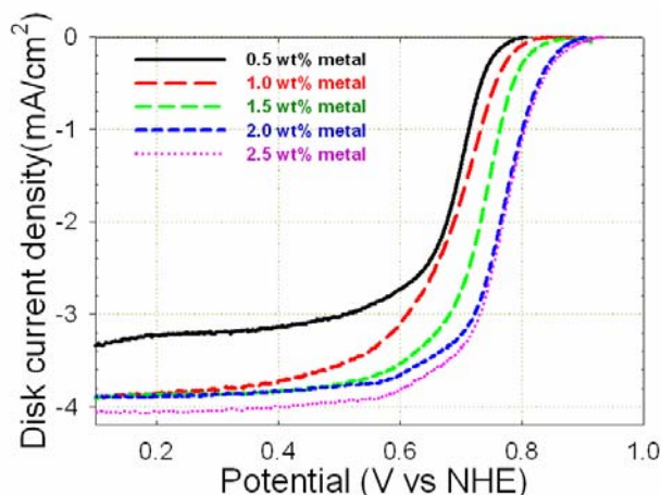
Figure 3. Effect of the metal content in the synthesis on ORR activity of various PANI-FeCo-C catalysts.
