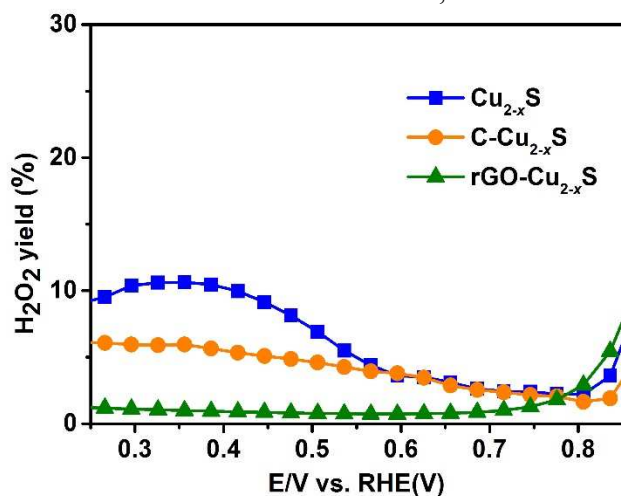
Figure 6. H 2 O 2 yield plots measured with the Cu 2-x S, C-Cu 2-x S and rGO-Cu 2-x S catalysts in O 2 -saturated 0.1 M NaOH at room temperature with rotation rate of 900 rpm.
