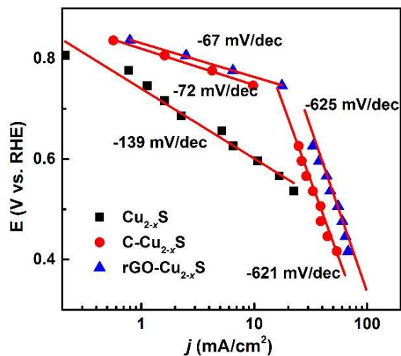
Figure 8. Tafel plots for the ORR on \text{Cu}_{2-x}\text{S} , \text{C-Cu}_{2-x}\text{S} and \text{rGO-Cu}_{2-x}\text{S} .
