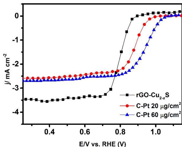
Figure 7. Polarization curves were measured in 0.1 M NaOH solution (room temperature, 900 rpm) for rGO-Cu 2-x S and C-Pt. The loading amount of Pt was 20 μg/cm 2 (red curve) and 60 μg/cm 2 (blue curve) respectively.
