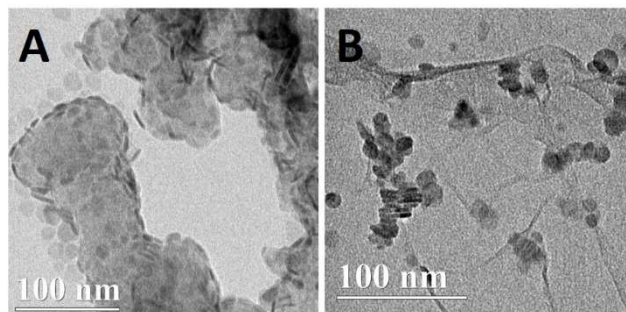
Figure 5. TEM images of \text{Cu}_{2-x}\text{S} nanoplates deposited on carbon black (C- \text{Cu}_{2-x}\text{S} , A) and reduced graphene oxide (rGO- \text{Cu}_{2-x}\text{S} , B).
