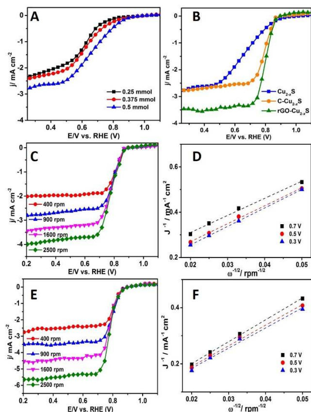
Figure 4. (A) ORR steady-state polarization curves of \text{Cu}_{2-x}\text{S} NCs synthesized using 0.25 mmol, 0.375 mmol and 0.5 mmol Cu precursors. (B) steady-state polarization curves for \text{Cu}_{2-x}\text{S} NCs, C- \text{Cu}_{2-x}\text{S} and rGO- \text{Cu}_{2-x}\text{S} . (C&E) ORR steady-state polarization curves for C- \text{Cu}_{2-x}\text{S} (C) and rGO- \text{Cu}_{2-x}\text{S} (E) with varying electrode rotation rates. (D&F) Koutecky-Levich plots of the ORR for C- \text{Cu}_{2-x}\text{S} (D) and rGO- \text{Cu}_{2-x}\text{S} (F). The measurements were performed in \text{O}_2 -saturated NaOH.
