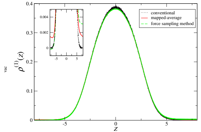
FIG. 1: Monte Carlo simulation results of the singlet density profiles obtained using uniform mapped-averaging (Eq. (20)), force sampling [12], and conventional histogram methods. Simulated system is a Lennard-Jones (LJ) fluid under the influence of parabolic external potential, \phi_1 = \epsilon(z/\sigma)^2 , where \sigma and \epsilon are the LJ size and energy parameters, respectively. Plotted quantities are in units such that \sigma = 1 . Inset figure shows the same curves but with the ordinate scale greatly expanded to show the behavior of the tails. Additional simulation details are provided in the Appendix.
